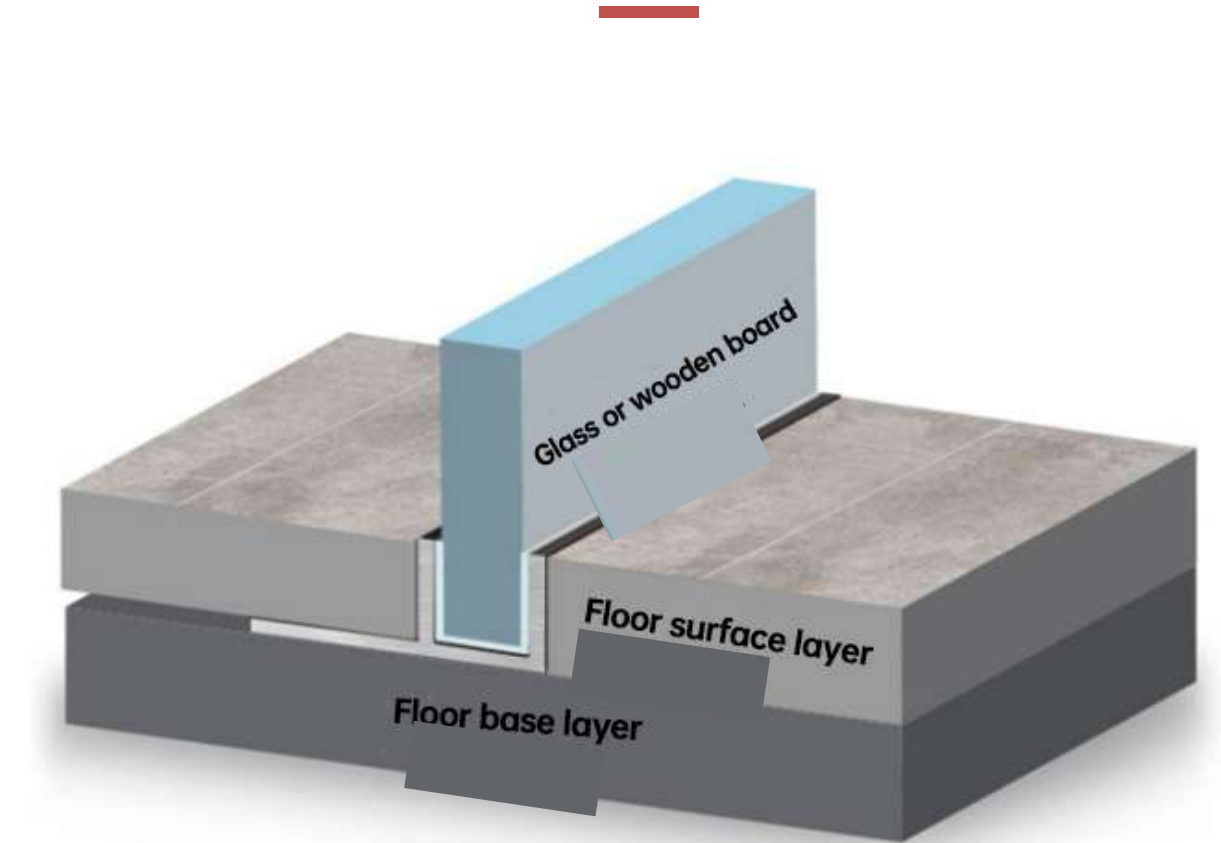
Flush transition construction method
