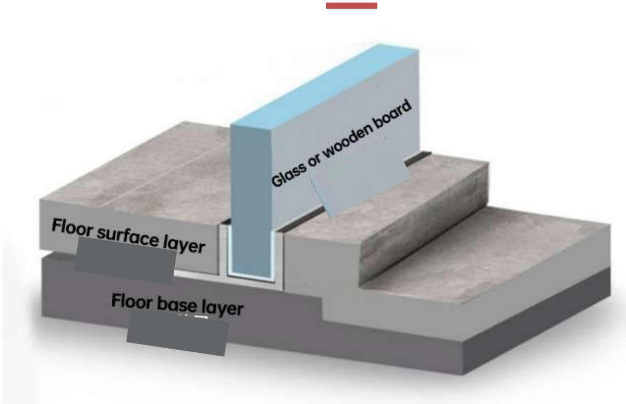
Construction method of sunken shower room
