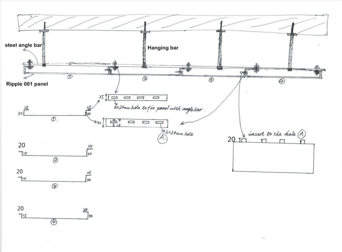
Hanging drawing
